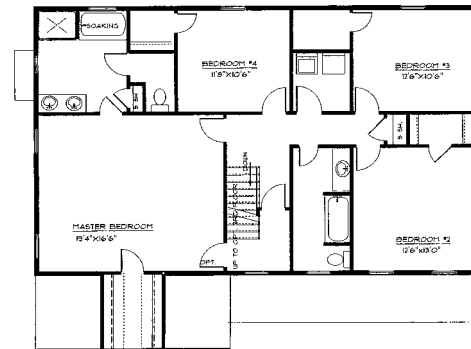
SECOND FLOOR PLAN - 1339 S.F.
