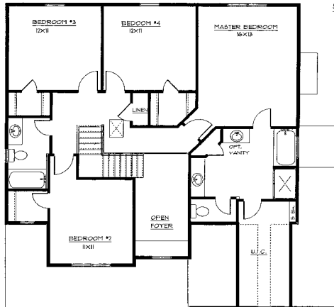
SECOND FLOOR PLAN W/4 BEDROOMS
