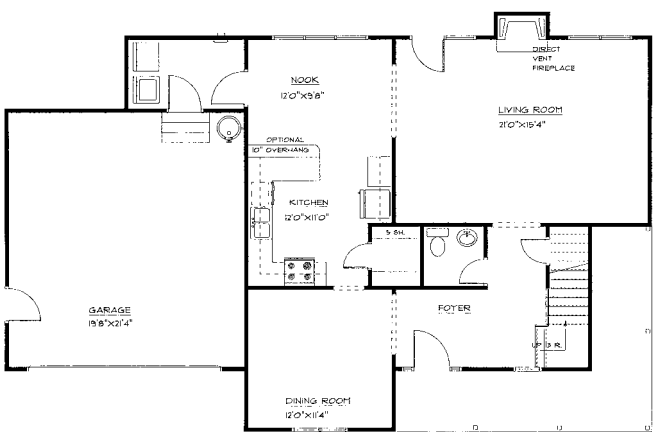
FIRST FLOOR PLAN - 1019 S.F. (FINISHED) - FRONT LOAD THE "BAYLOR" MODEL
